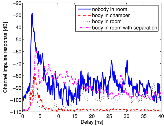
Figure 10- The average channel impulse responses comparing the scenarios in the chamber and in the classroom, when the Tx is at level 1 position 2
