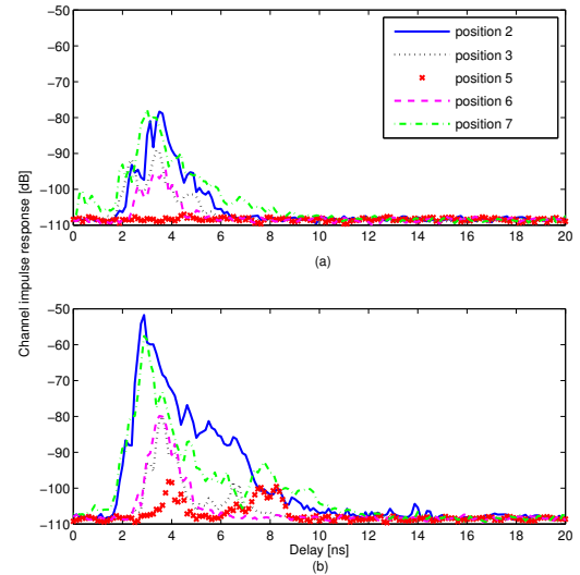
Figure 6- Average channel impulse responses for the 1 st set level 1: (a) without separation and (b) with separation
