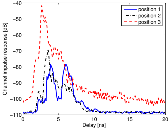
Figure 9- The average channel impulse responses in the 2 nd set
