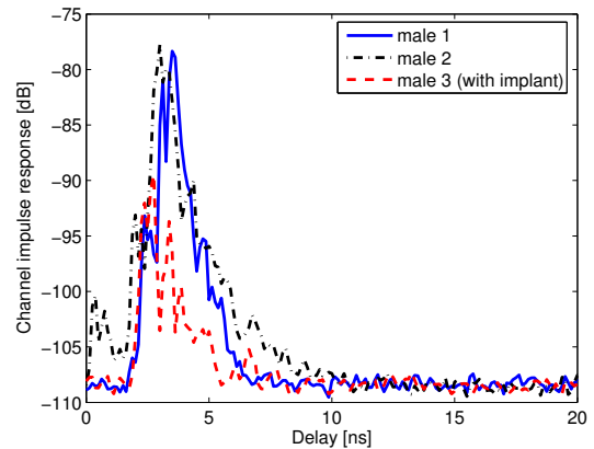
Figure 7- Average channel impulse responses in the 1 st set (level 1, position 2) for three male subjects.
