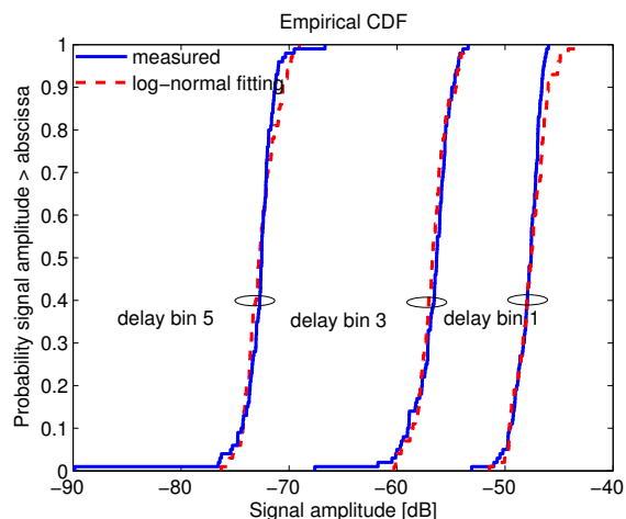
Figure 12- The amplitude distribution of the delay bins 1, 3, and 5 in the 1 st set (without separation) when the Tx is at level 1, position 1, and the log-normal distribution fitting
