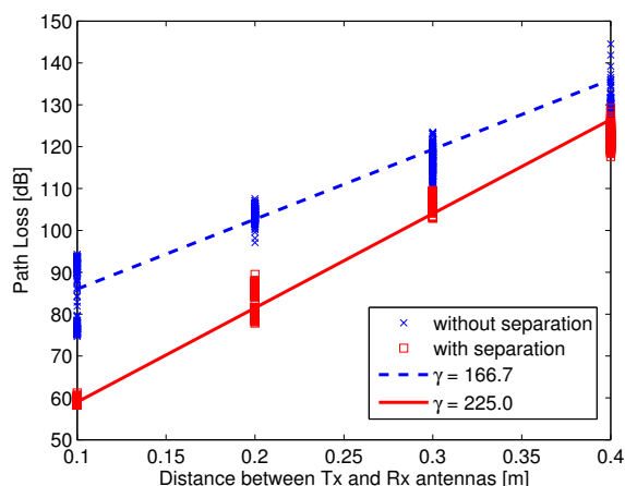
Figure 13- The path loss versus distance for the 1 st set with and without separation
