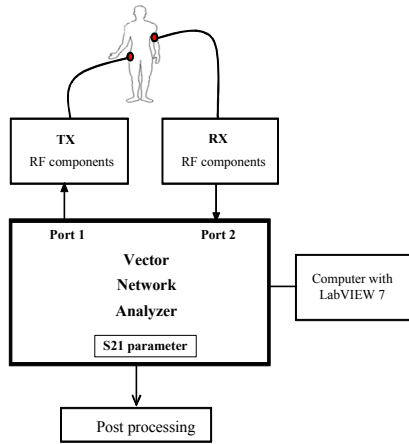
Figure 2- Frequency domain measurement using VNA
