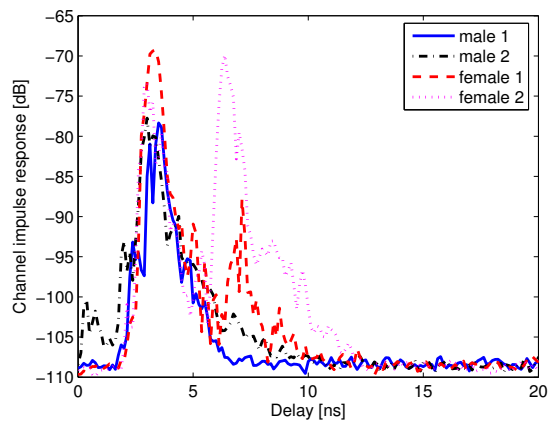
Figure 8- The average channel impulse responses in the 1 st set (level 1, position 2) comparing male and female subjects.
